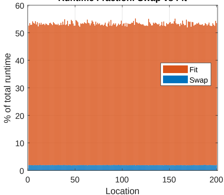
Runtime Fraction: Swap vs Fit
